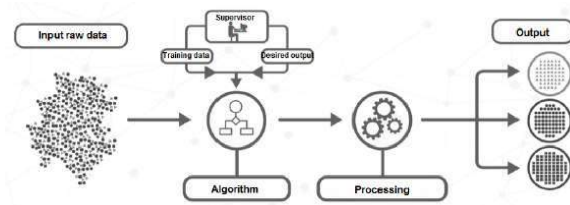
Figure 1.4: Supervised learning
